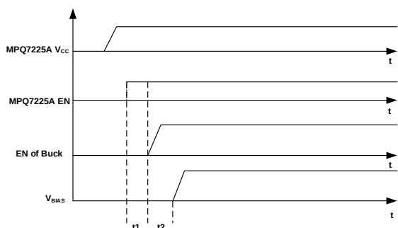
Figure 9: Start-Up Sequence
