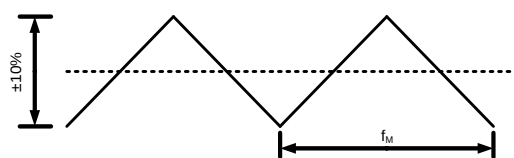
Figure 10: Frequency Spread Spectrum
