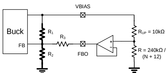
Figure 22: AFC Modulator Network with FBO Open Protection
