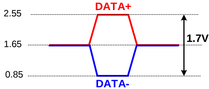
Figure 1: Differential Interface Timing
