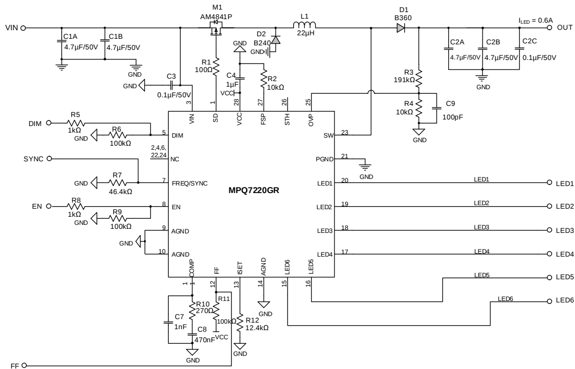
Figure 4: I_{SET} = 100\text{mA} , f_{SW} = 470\text{kHz} , Application Circuit for TSSOP-28 Package
