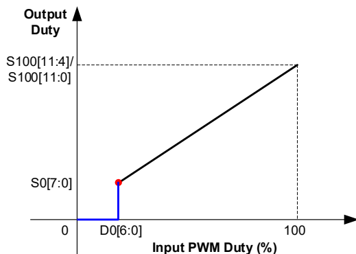
Figure 2: Minimum Speed of Starting Duty
