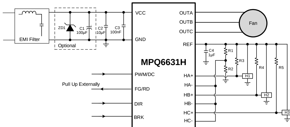
Figure 14: Typical Application Circuit (Triple Hall-Effect Sensor Application)
