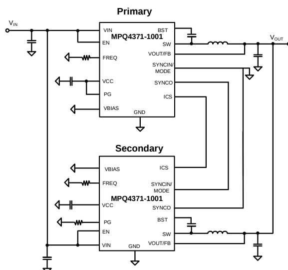
Figure 8: Dual-Phase Configuration
