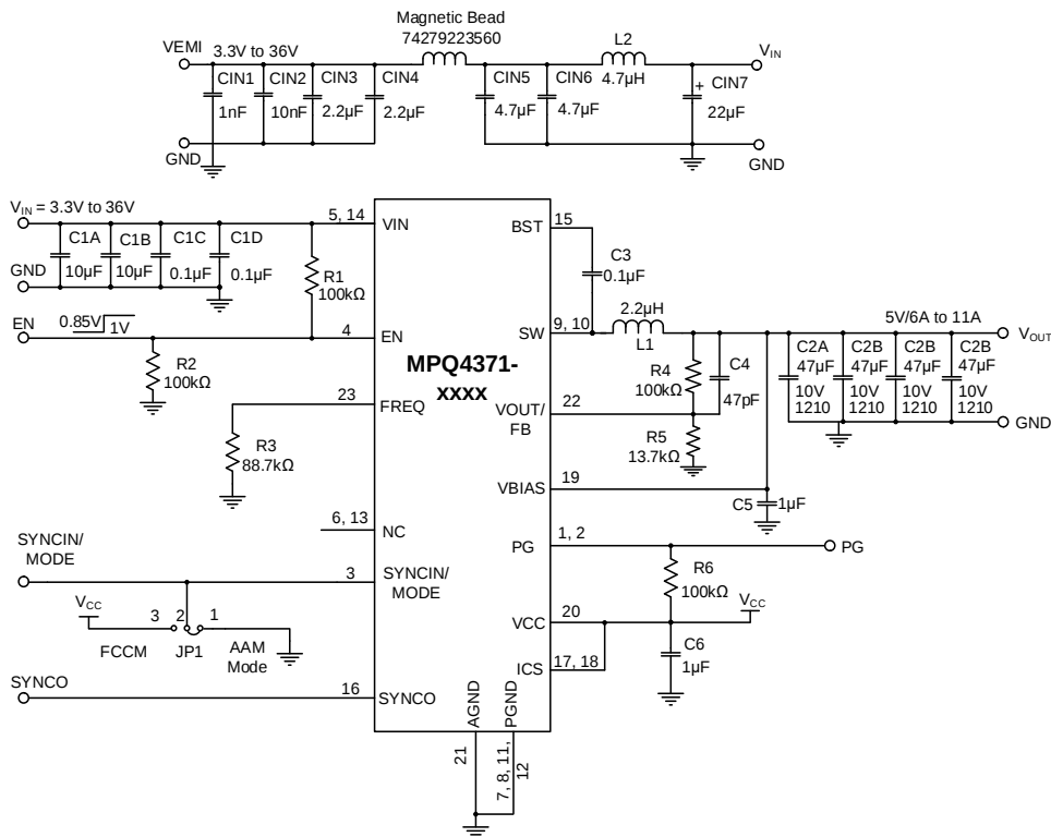
Figure 20: Typical Application Circuit (Single-Phase, V_{OUT} Adjustable for the MPQ4371-xxxx, V_{OUT} = 5V , f_{sw} = 410kHz with EMI Filter)
