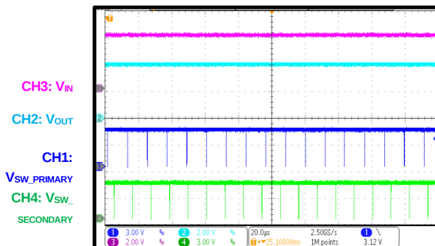
Dropout Operation
