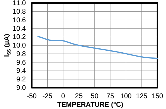
Soft-Start Current vs. Temperature
