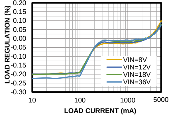
Load Regulation
