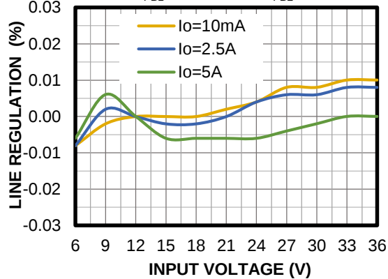
Line Regulation
