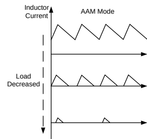
Figure 3: AAM Operation
