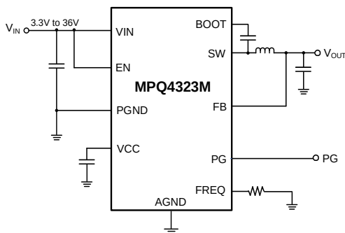
Typical Application (Fixed Output)
