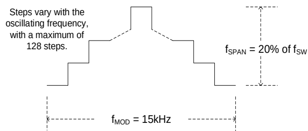
Figure 4: Frequency Spread Spectrum
