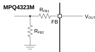
Figure 7: FB Divider Network (Fixed-Output Version)
