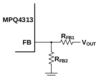
Figure 8: Feedback Network
