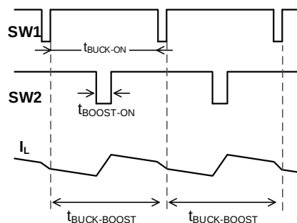
Figure 5: Buck-Boost Waveform
