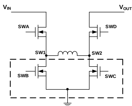
Figure 3: Buck-Boost Topology
