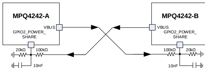
Figure 15: GPIO2 Power Share Connection Between Two MPQ4242s
