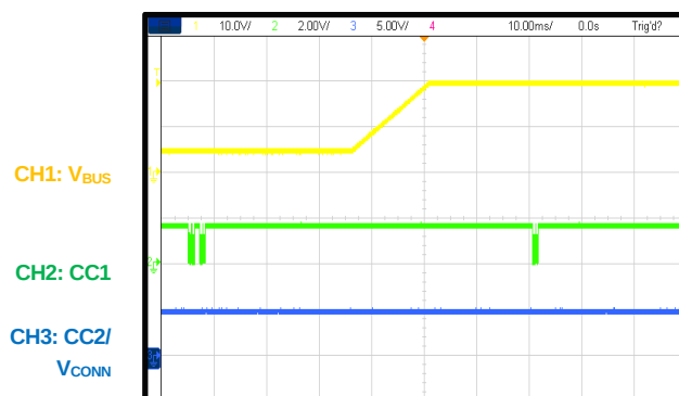
PDO Transition 5V PDO to 20V PDO
