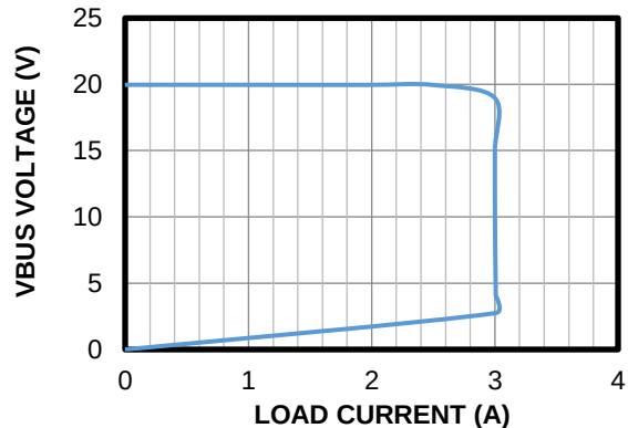
VBUS Voltage vs. Load Current
