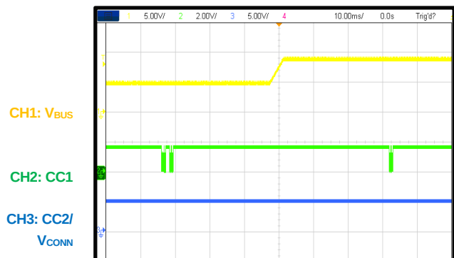
PDO Transition
