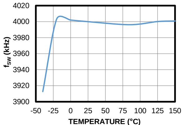
f_{SW} vs. Temperature (CBh, bits[1:0] = 2'b11)
