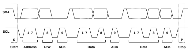
Figure 7: A Complete Data Transfer
