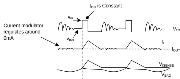
Figure 3: Light-Load Operation
