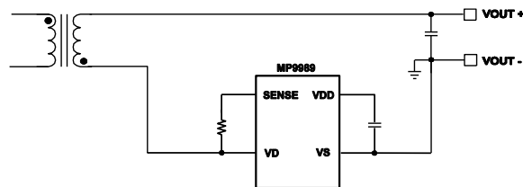
Figure 3: Low-Side Rectification
