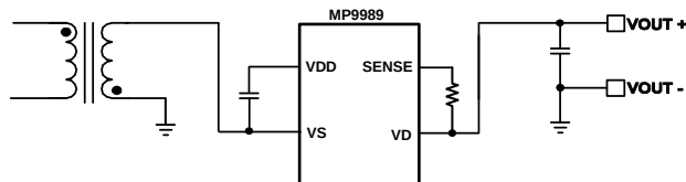
Figure 4: High-Side Rectification
