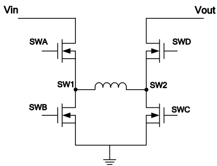
Figure 3: Buck-Boost Topology
