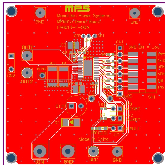
Figure 3: Recommended PCB Layout (MP6613GF)
