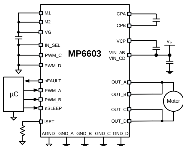
Mono DC Motor Application with Parallel Mode
