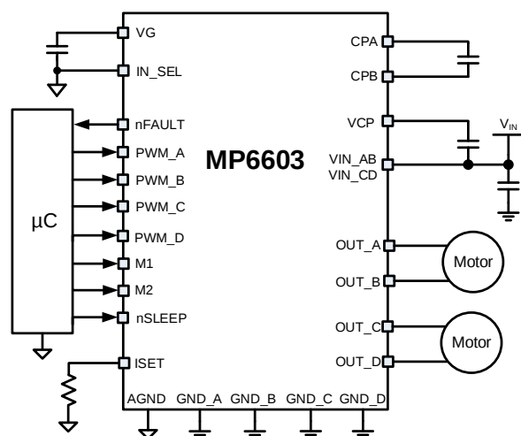
Dual DC Motor Application
