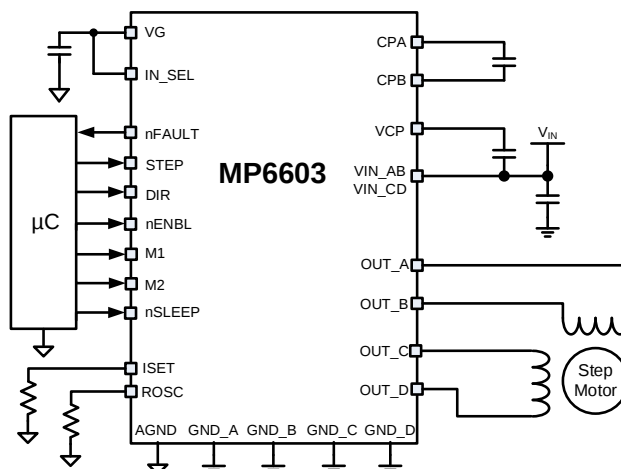
Stepper Motor Application with Indexer Input
