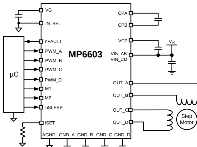
Stepper Motor Application with PWM Input
