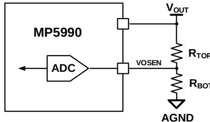
Figure 22: Output Voltage Sense Circuit Design
