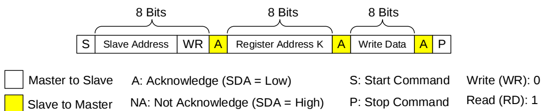
Figure 6: I 2 C Write Example (Write Single Register)
