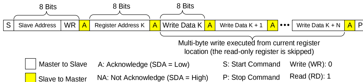
Figure 7: I 2 C Write Example (Write Multi-Register)
