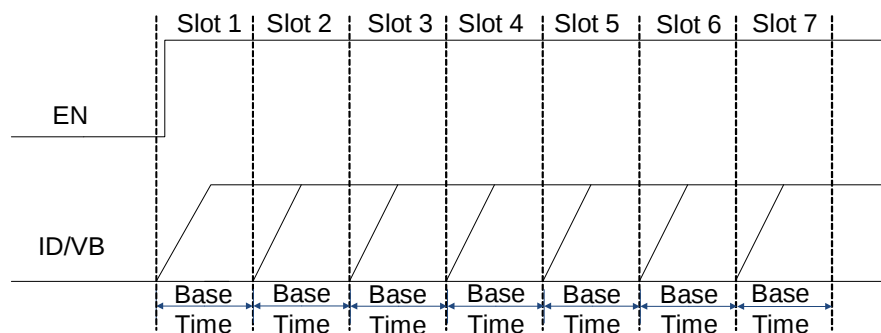
Figure 12: Time Delays
