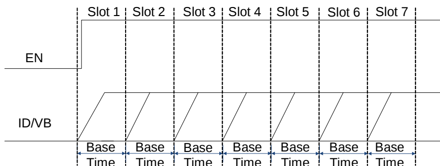
Figure 9: Time Delays
