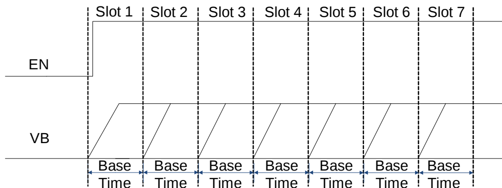
Figure 11: Time Delays
