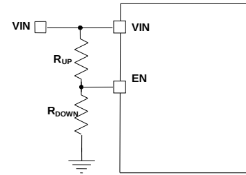
Figure 7: Adjustable UVLO via the EN Divider
