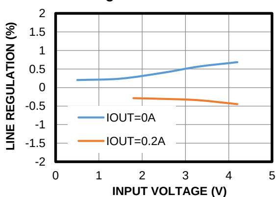
Line Regulation
