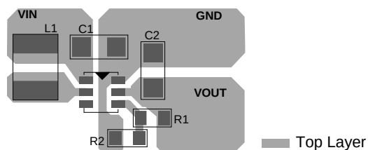
Figure 3: Recommended PCB Layout
