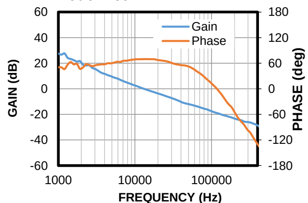
Bode Plot
