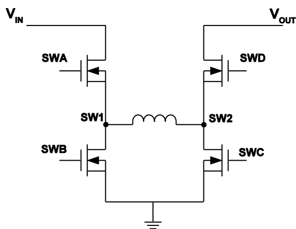
Figure 2: Buck-Boost Topology
