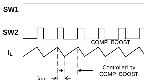
Figure 5: Boost Waveform
