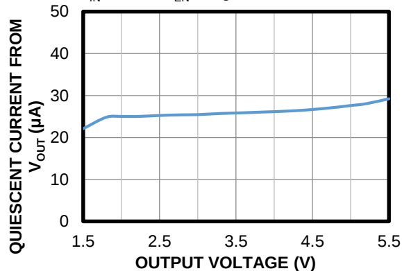
Quiescent Current From V_{OUT}
