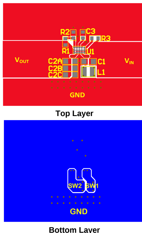
Figure 3: Recommended PCB Layout
