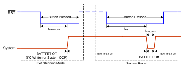
Figure 6: RST Timing
