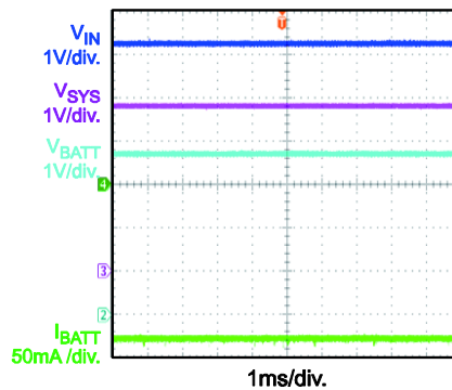
Input Current Limit based PPM
