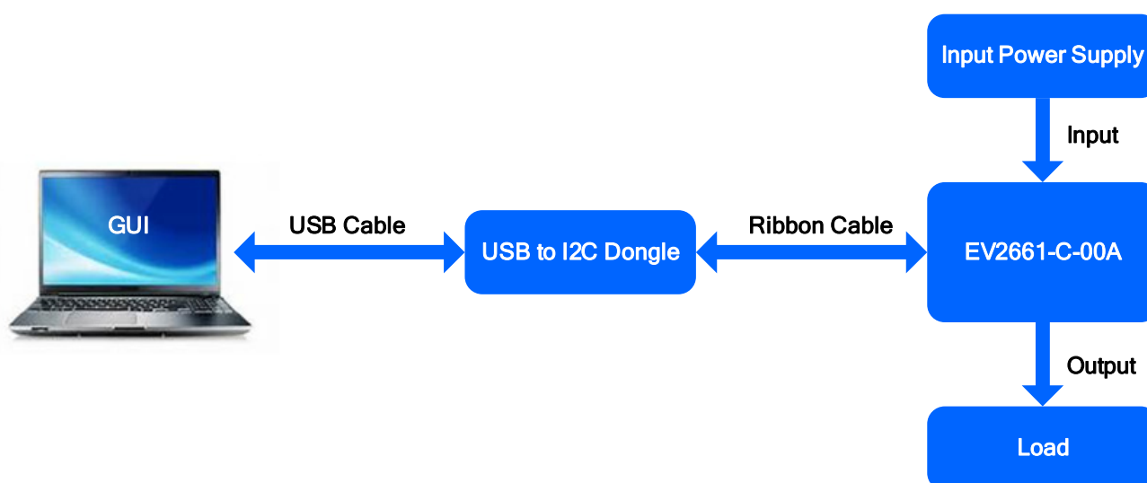
EVKT-2661 Evaluation Kit Set-Up
