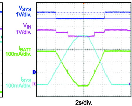
Input Current Limit based PPM
