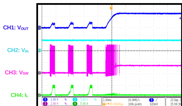
Short-Circuit Recovery
