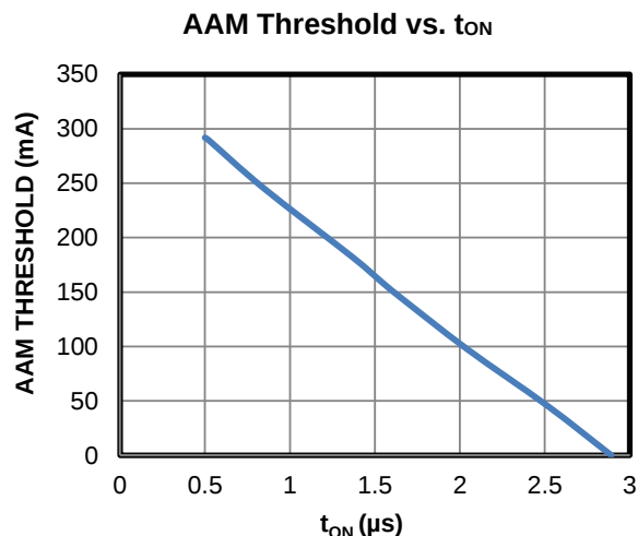
Figure 8: AAM Threshold Decreases as t_{ON} Increases
