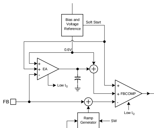
Figure 2: Operation Blocks in Sleep Mode
