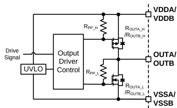
Figure 9: Output Stage
