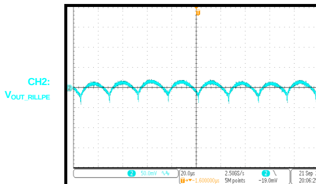
Output Ripple
