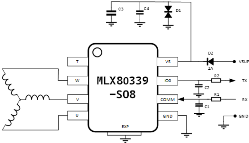
Figure 14: Application circuit
