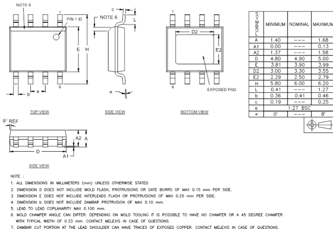
Figure 3: Package Drawing SOIC8 with exposed pad
