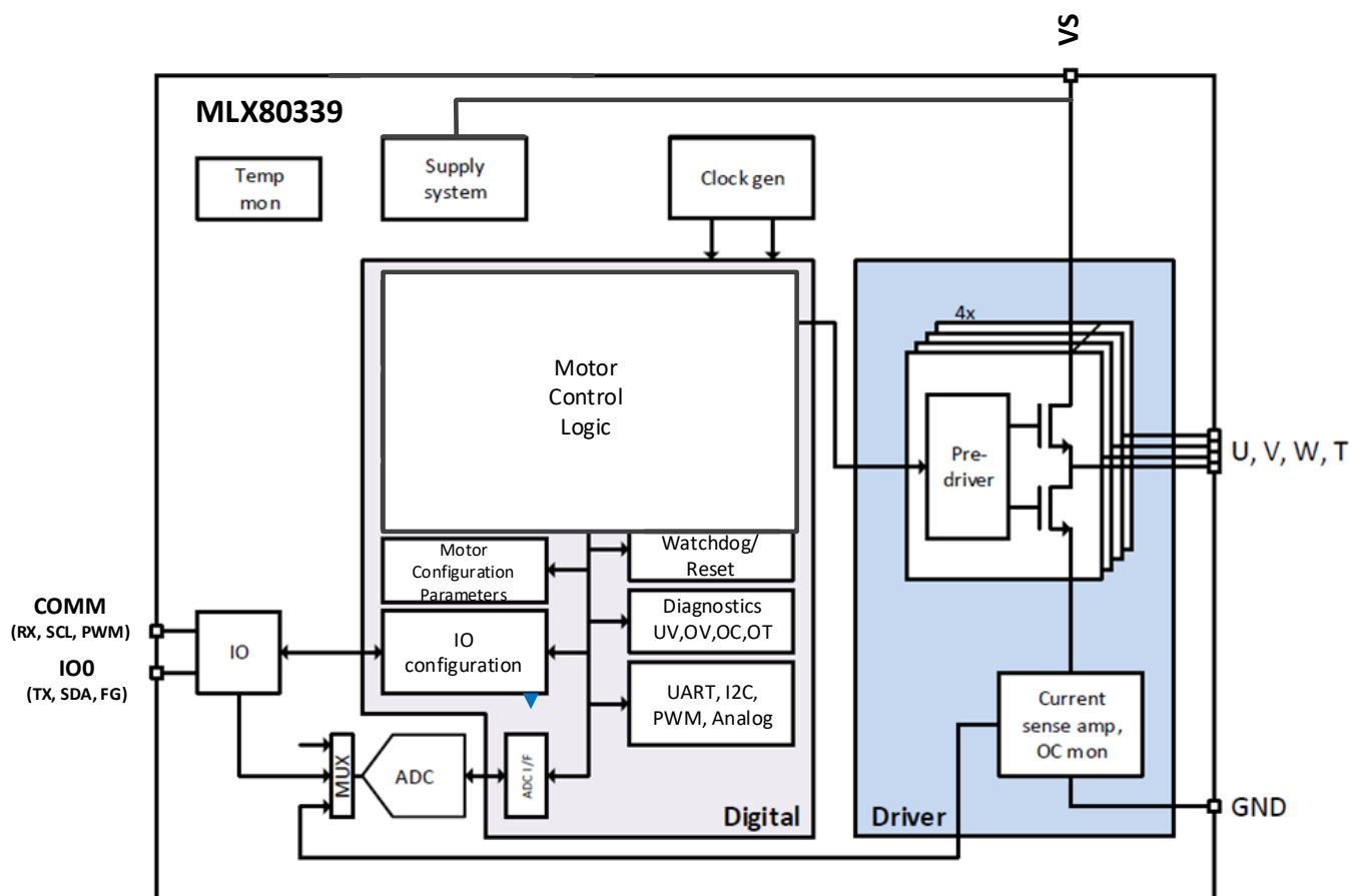
Figure 2: IC Block diagram
