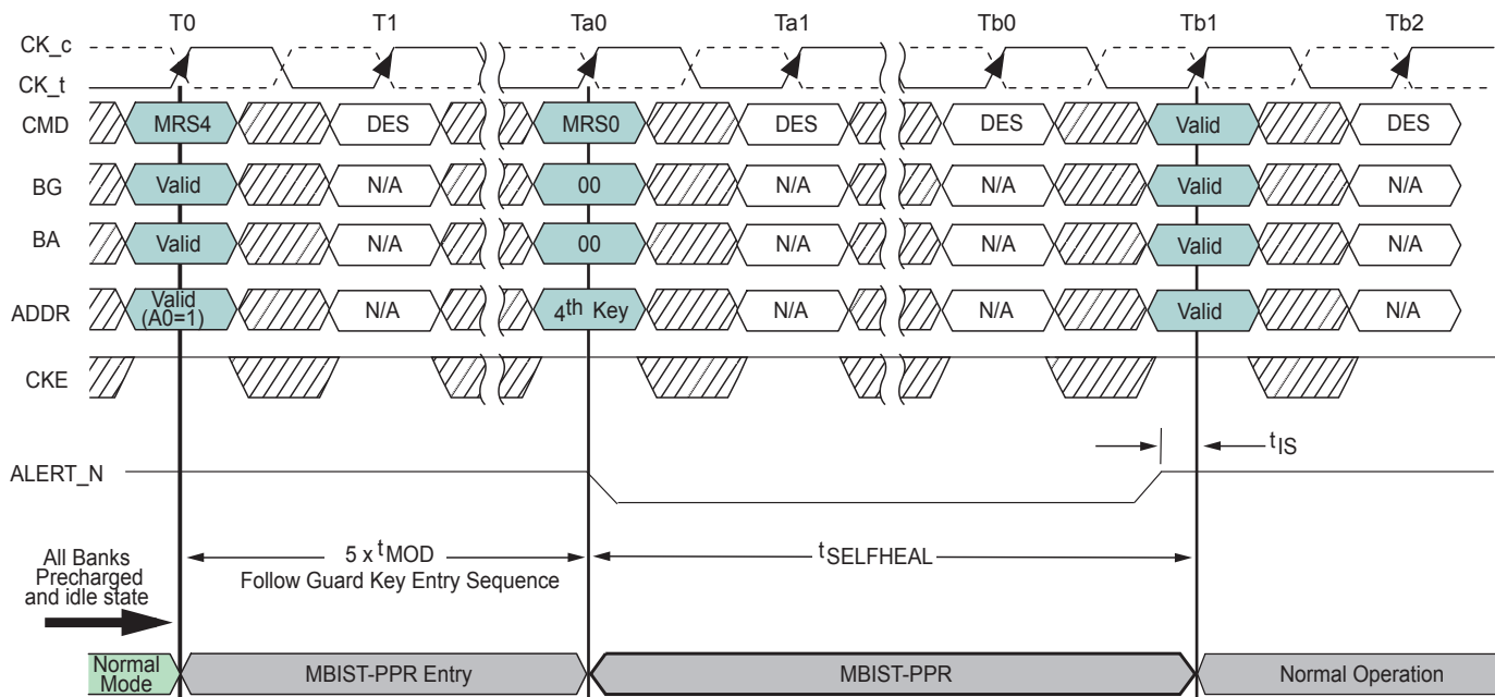
Figure 80: MBIST-PPR Sequence
