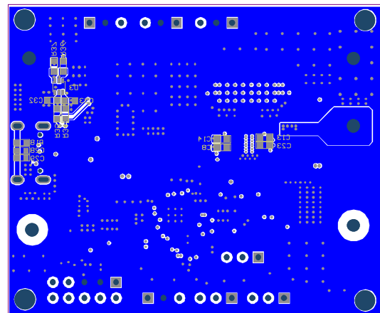
Figure 21: Bottom Layer
