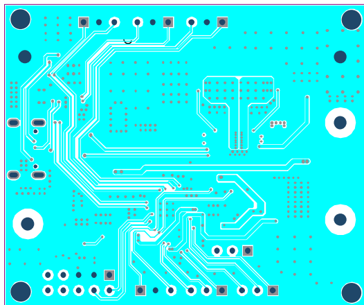
Figure 20: Mid-Layer 2
