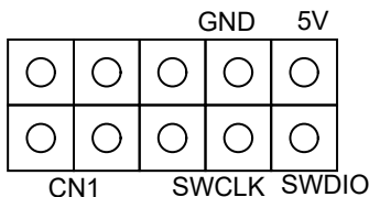
Figure 10: SWD Port on the MPF52002
