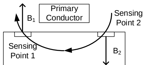
Figure 3: Sensor's Cross-Section
