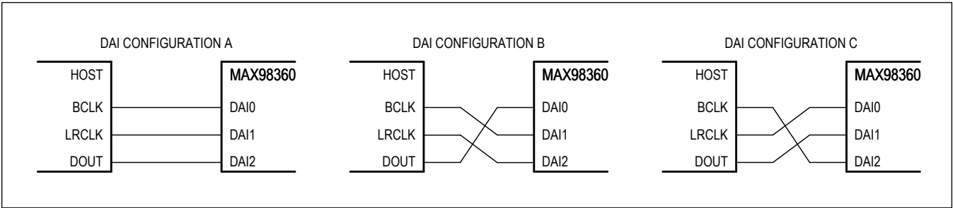
Figure 1. DAI Connections
