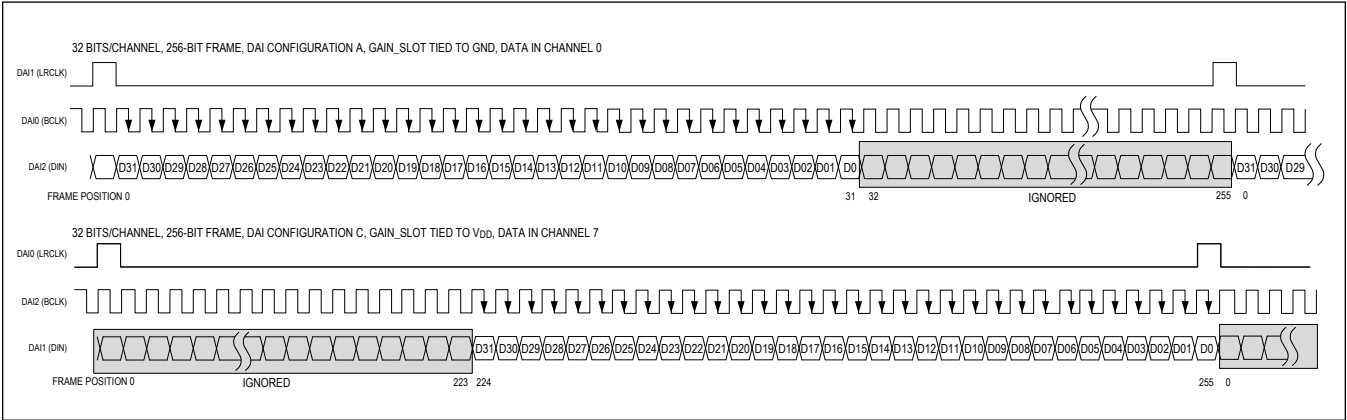
Figure 11. MAX98360B and MAX98360D TDM Protocol, 32-Bit Resolution
