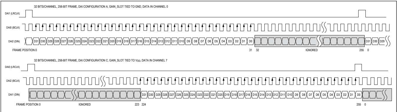
Figure 9. MAX98360A and MAX98360C TDM Protocol, 32-Bit Resolution
