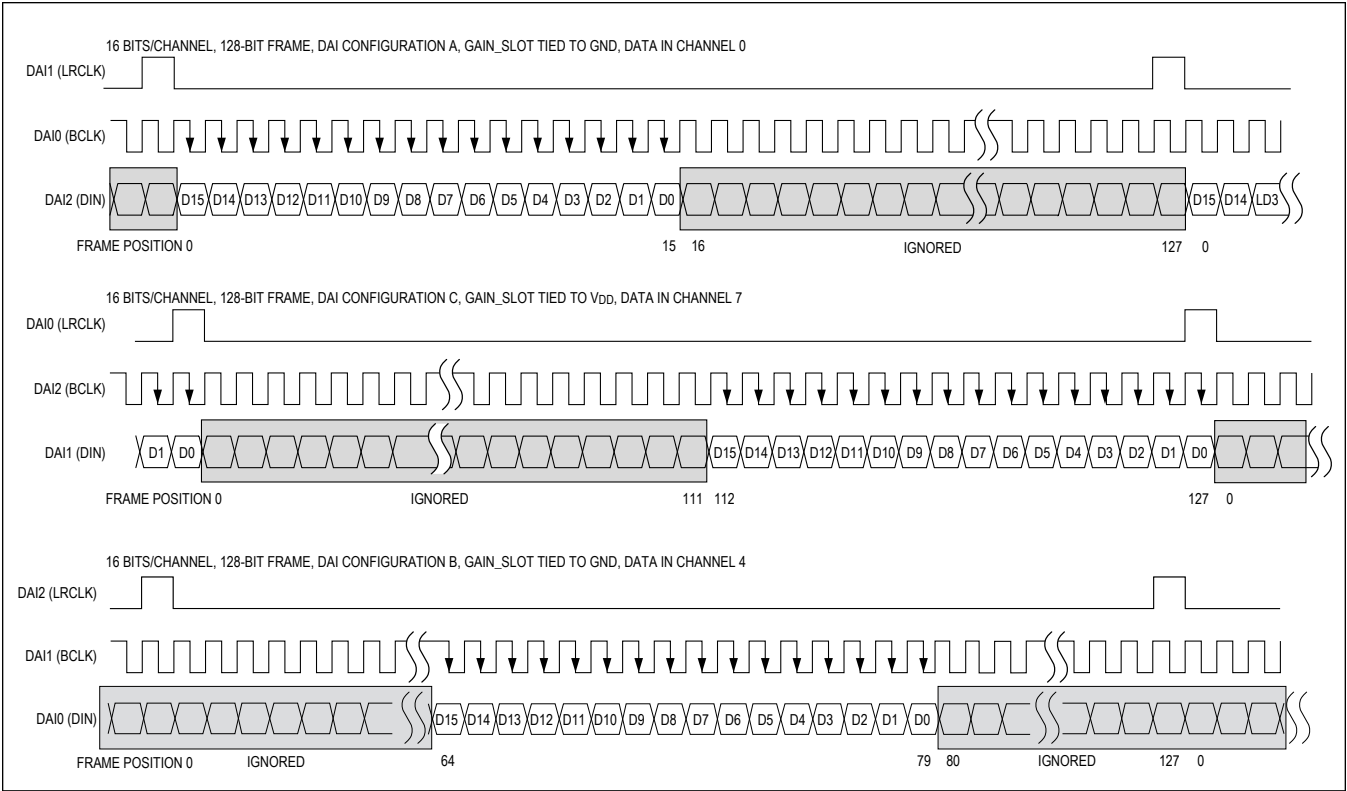
Figure 10. MAX98360B and MAX98360D TDM Protocol, 16-Bit Resolution
