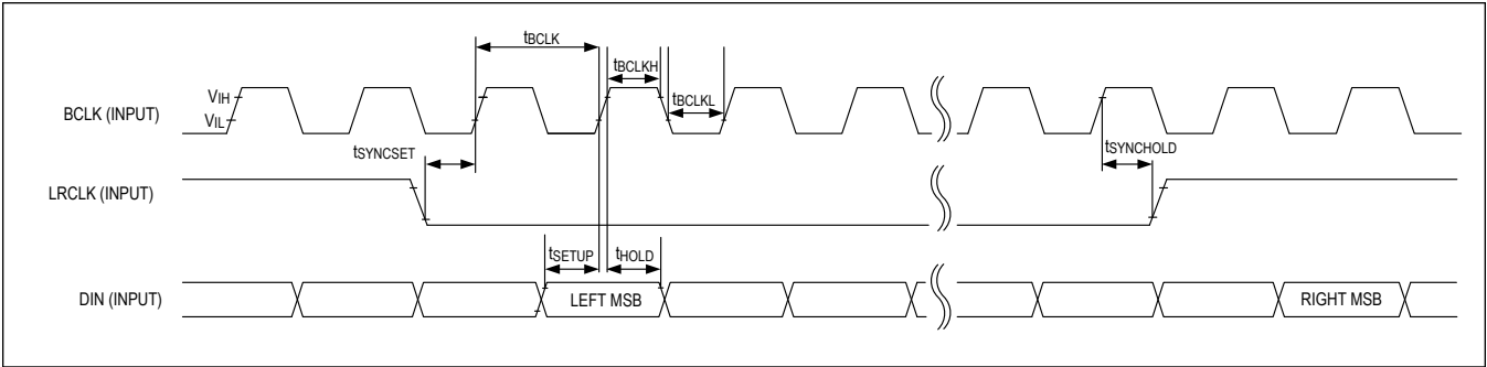
Figure 6. I²S Timing Diagram (MAX98360A and MAX98360C)
