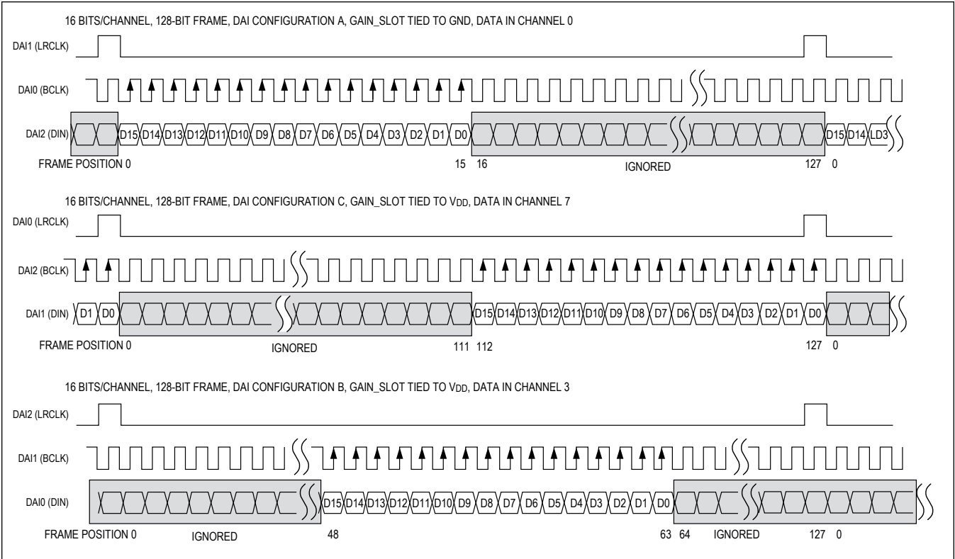
Figure 8. MAX98360A and MAX98360C TDM Protocol, 16-Bit Resolution
