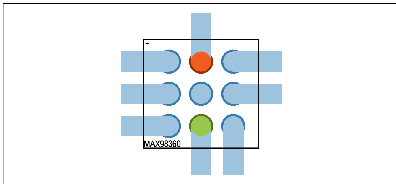
Figure 15. GAIN_SLOT Unconnected (Gain is 9dB in I 2 S and Left-Justified Modes)
