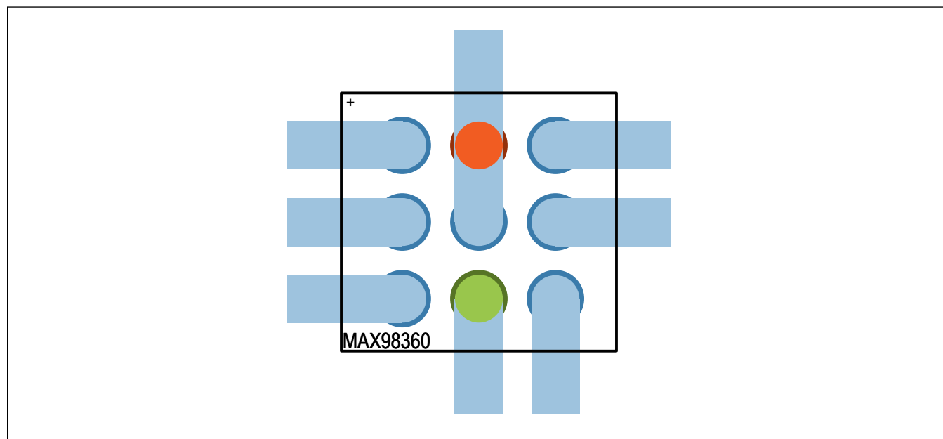
Figure 14. GAIN_SLOT Tied to V DD (Gain is 6dB in I 2 S and Left-Justified Modes)
