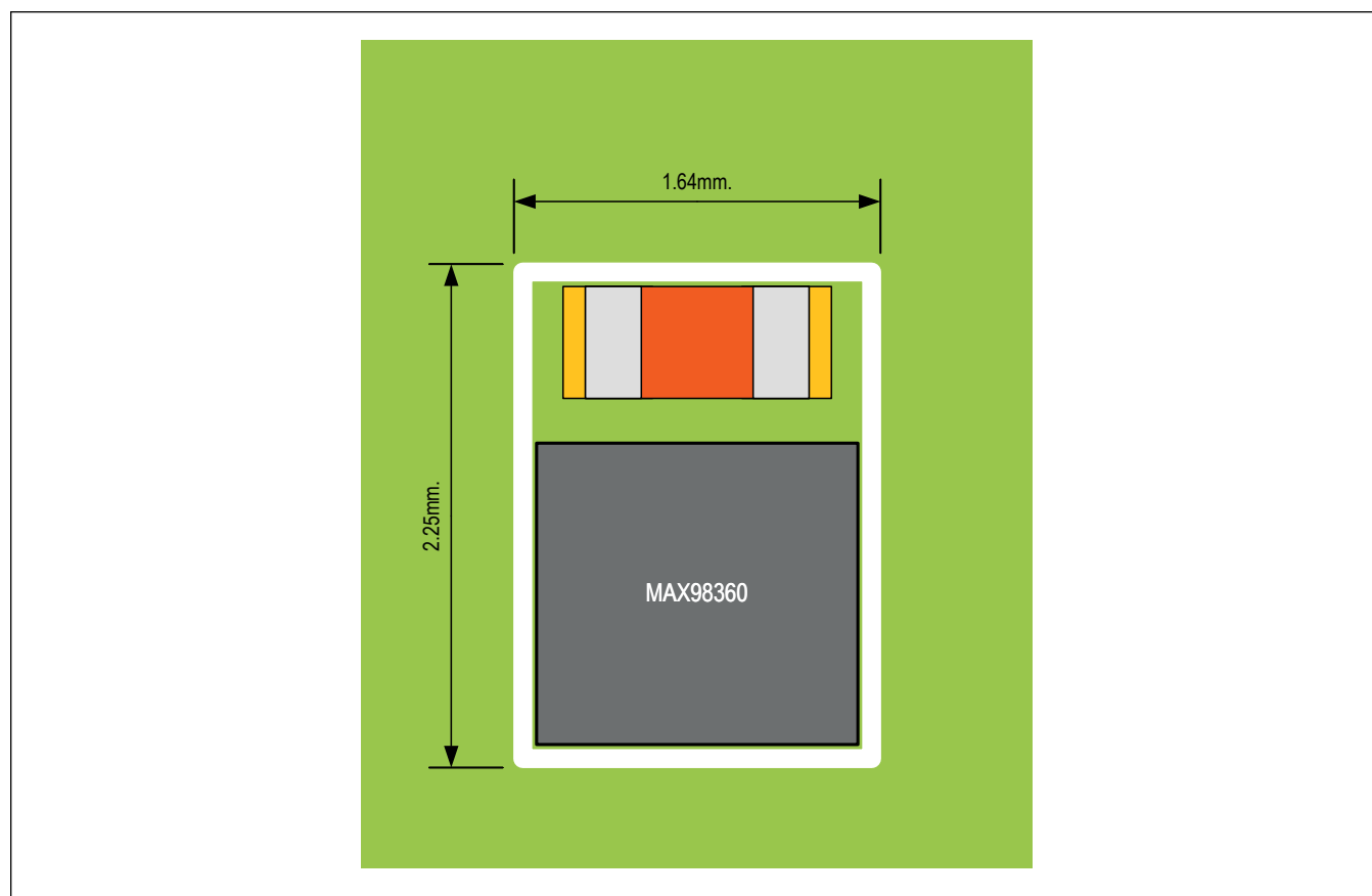
Figure 13. Solution Size
