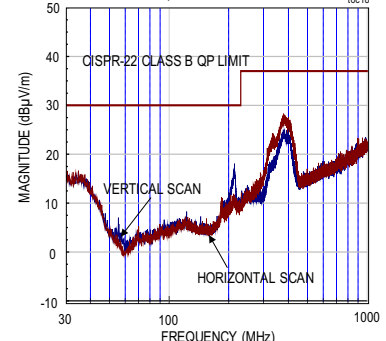
RADIATED EMISSIONS PLOT 5V OUTPUT, 4.25A LOAD CURRENT
