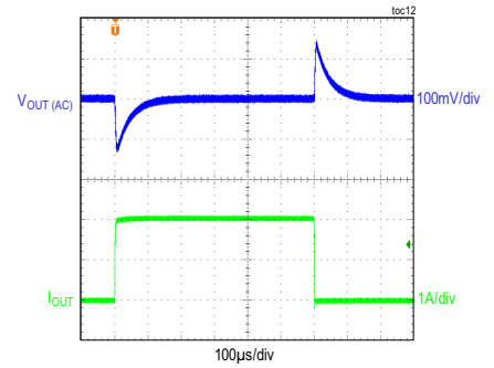
LOAD TRANSIENT BETWEEN 0A AND 2A
