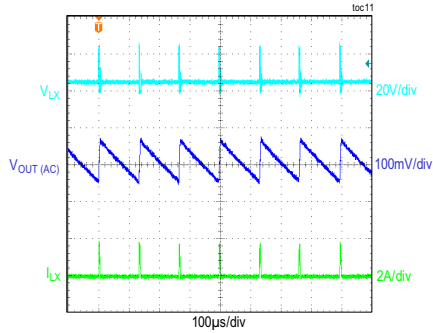
STEADY-STATE PERFORMANCE
