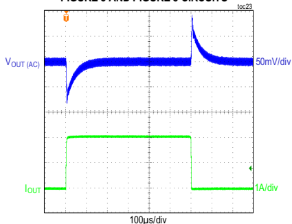
LOAD TRANSIENT BETWEEN 0A AND 2A FIGURE 3 AND FIGURE 5 CIRCUITS
