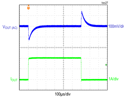
LOAD TRANSIENT BETWEEN 0A AND 2A FIGURE 4 AND FIGURE 6 CIRCUITS
