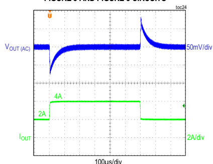
LOAD TRANSIENT BETWEEN 2A AND 4A FIGURE 3 AND FIGURE 5 CIRCUITS
