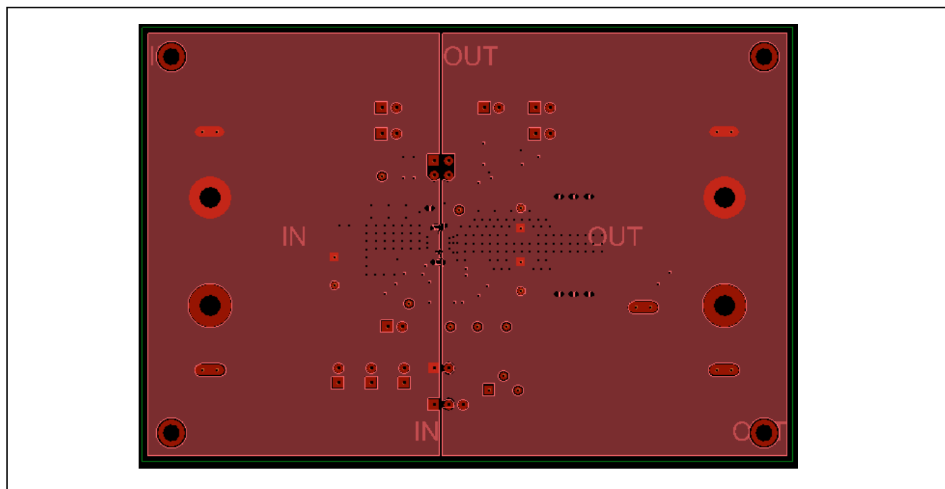
Figure 5. PCB Layout (Solder Side)
