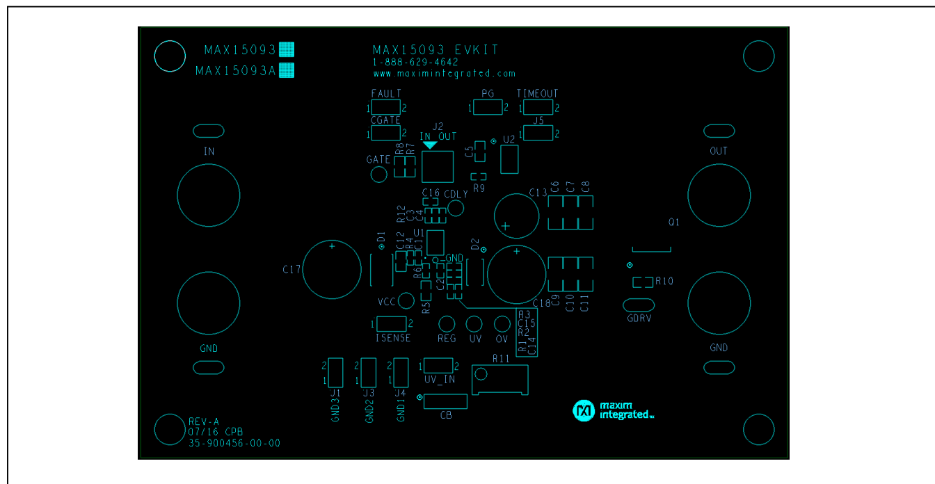
Figure 1. Component Placement Guide (Component Side)
