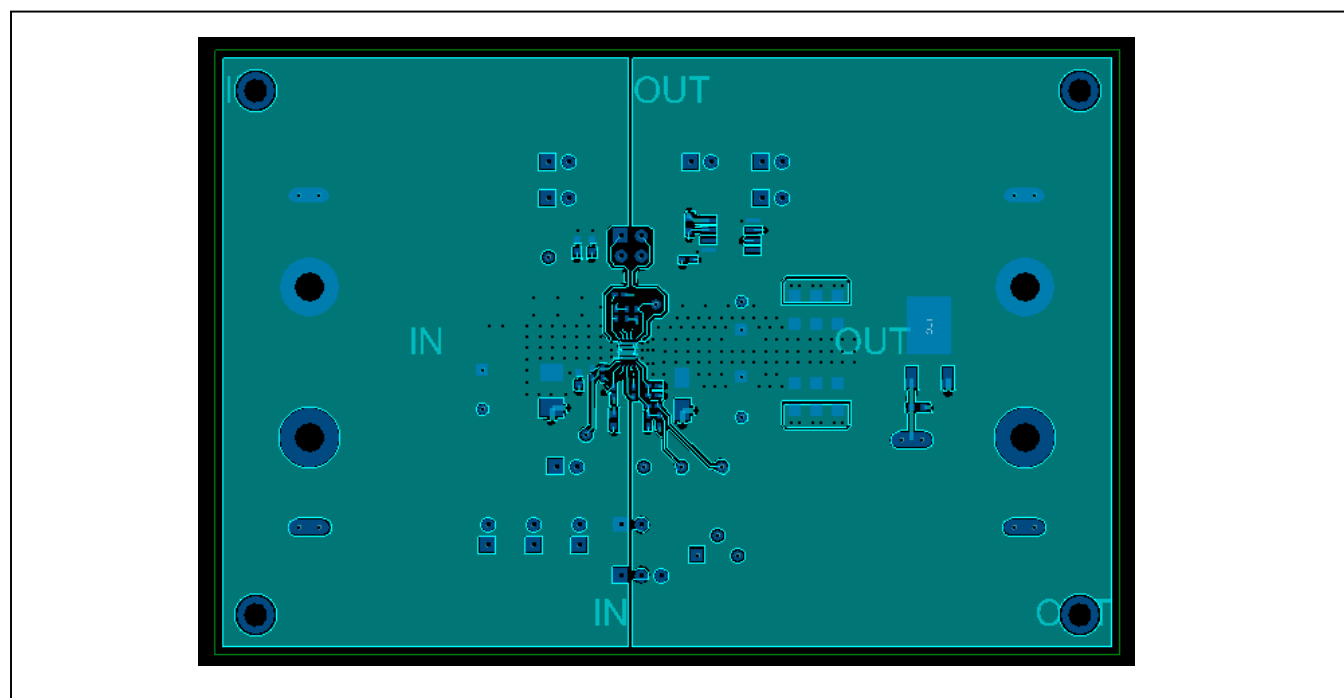
Figure 2. PCB Layout (Component Side)
