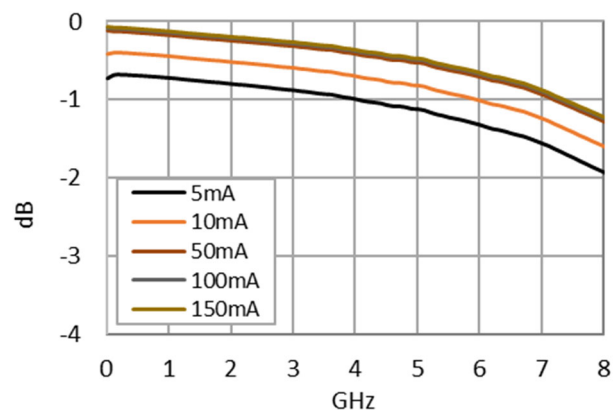
ANT Return Loss in RX ON state over Bias Current
