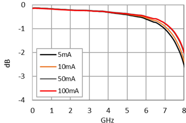
ANT to TX Insertion Loss over RX Bias Current
