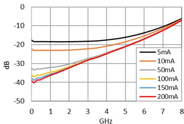
TX Return Loss in TX ON state over TX Bias Current
