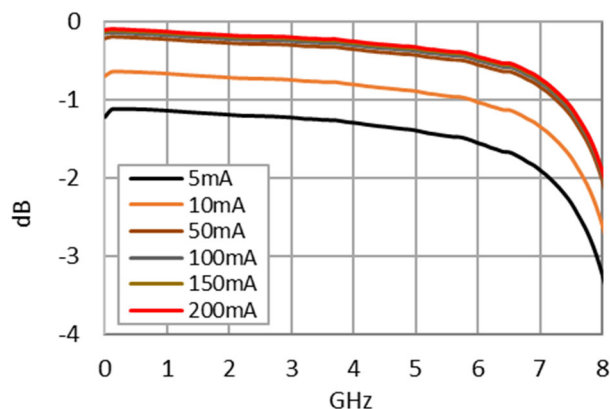
ANT Return Loss in TX ON state over TX Bias Current
