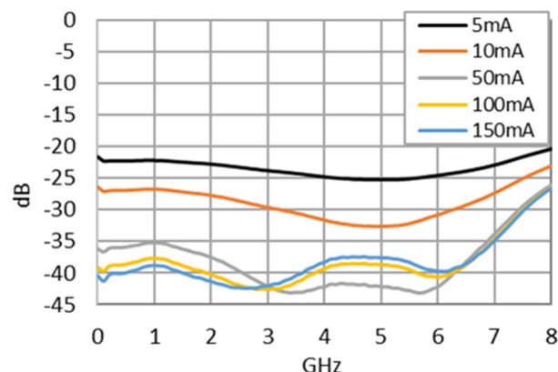
RX Return Loss in RX ON state over Bias Current
