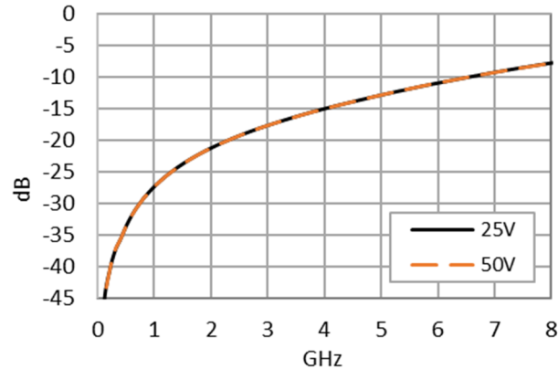
ANT to TX Isolation over TX Reverse Bias Voltage
