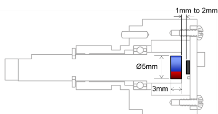
Figure 5: Potentiometer-Like Assembly
