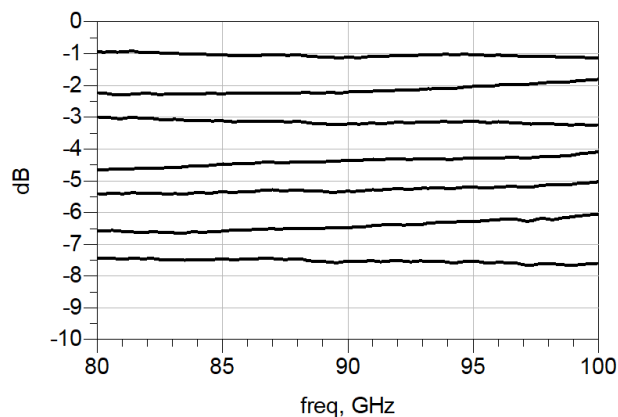
Relative Attenuation
