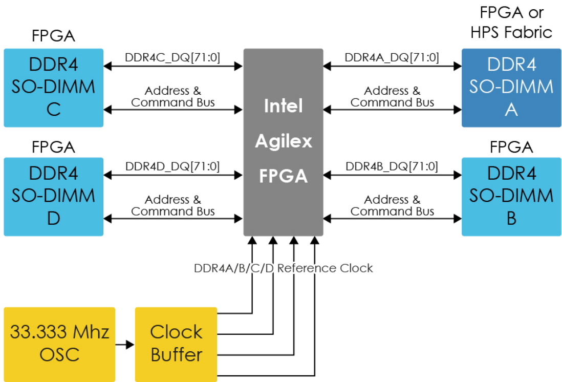
Figure 2-22 Connection between the DDR4 and Agilex FPGA
