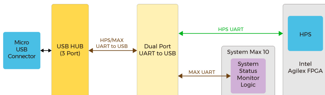
Figure 2-27 The UART interface on the board
