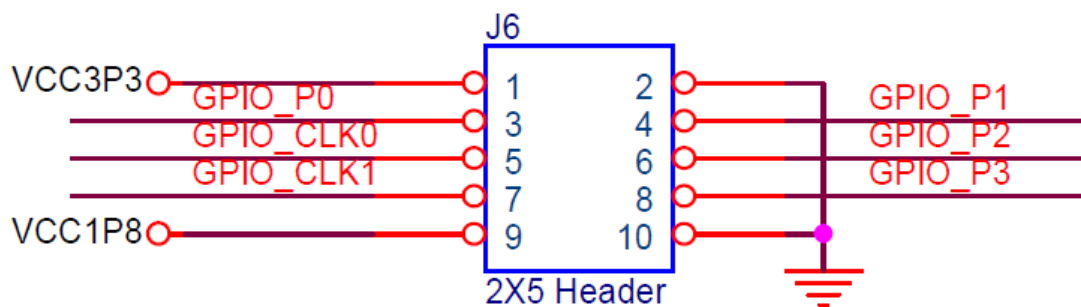
Figure 2-19 Pin-out of 2x5 expansion header
