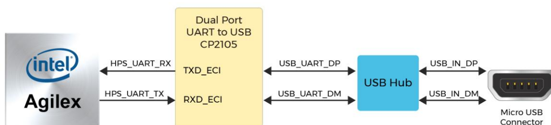
Figure 2-28 Connections between the HPS of Apollo Agilex and FT232R Chip
