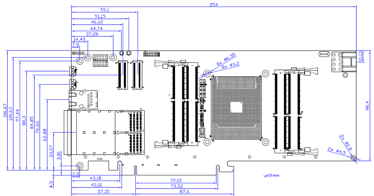
Figure 1-6 Mechanical layout
