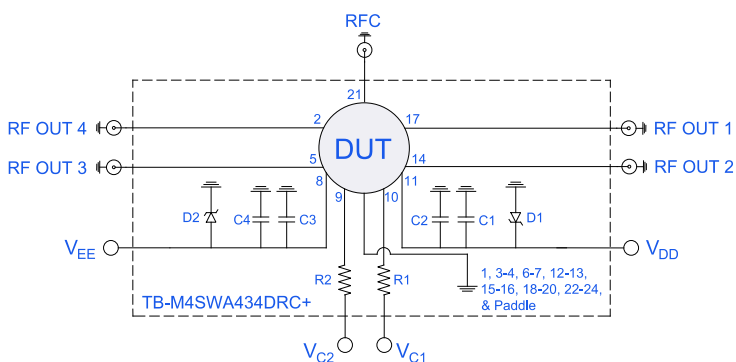
Figure 2. M4SWA4-34DR+ Characterization and Application Circuit
