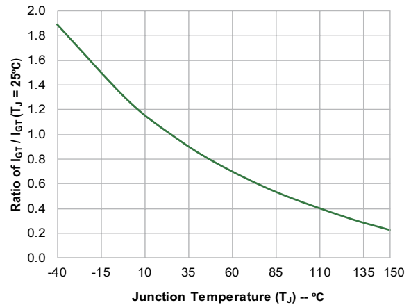
Figure 2: Normalized DC gate trigger current for Quadrants I, II, and III vs Junction Temperature
