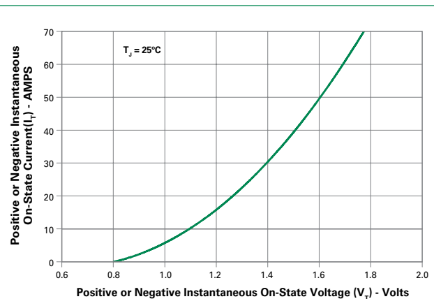
Figure 6: On-State Current vs. On-State Voltage (Typical)
