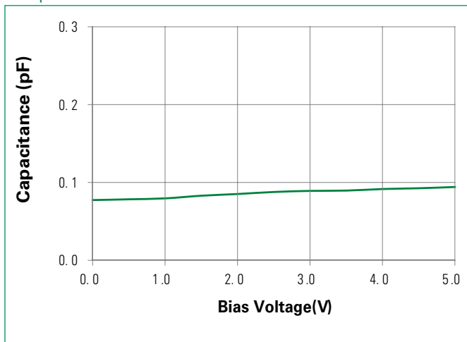
Figure 2. Capacitance vs. Reverse Bias Sub-0.1 pF silicon-based ESD protection
