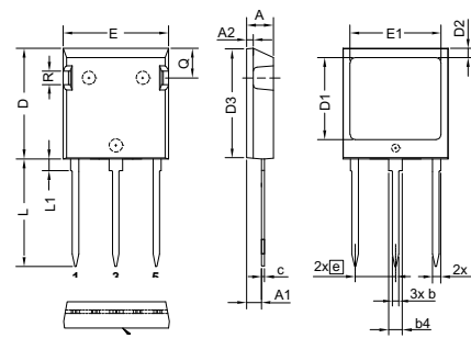
X024b ISOPLUS i4-PAC™ Weight = 5.5 g
