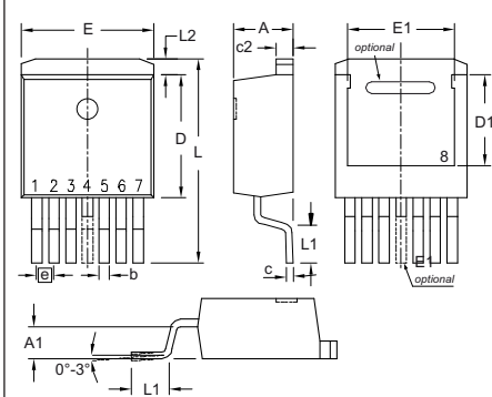
X012b TO-263 (7) c) middle leg cut Weight = 2.5 g
