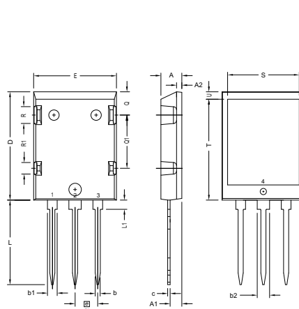
X022a ISOPLUS264™ Weight = 7.5 g
