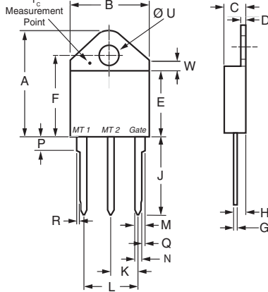
L002 TO-218AC Weight = 5 g
