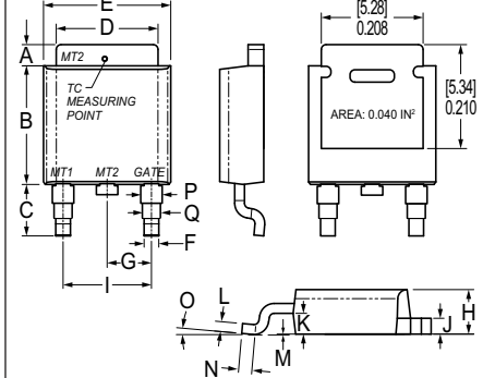
L004 TO-252AA Weight = 0.3 g
