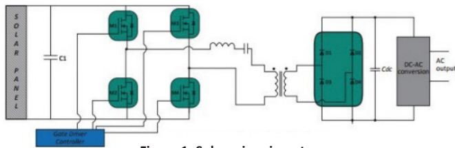
Figure 1: Solar micro-inverter
