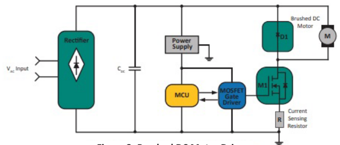
Figure 2: Brushed DC Motor Drive
