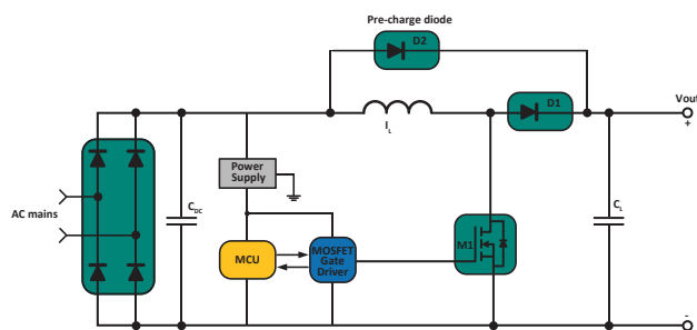
Figure 3: Power Factor Correction (PFC) circuit
