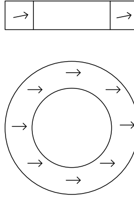
Figure 13 Magnetization tilt
