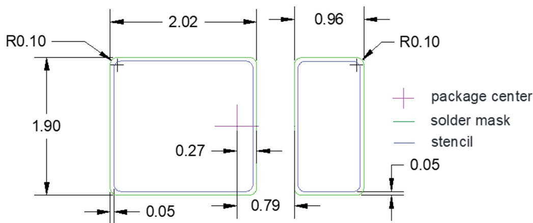
Figure 9. Recommended PCB solder pad layout for LUXEON 2835 Commercial Visual Consistency
