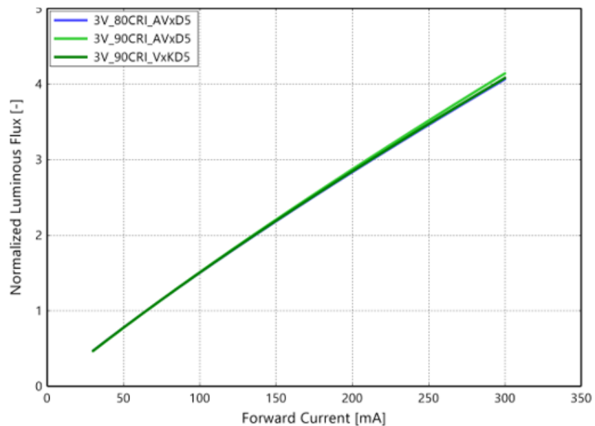
Figure 3b. Typical normalized luminous flux vs. forward current for LUXEON 2835S 3V at T j =25°C
