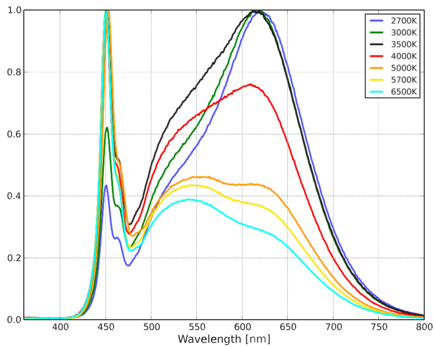
Figure 2b. Typical normalized power vs. wavelength for 90CRI LUXEON 2835 Commercial Visual Consistency at specified test current, T_j=25^{\circ}\text{C}
