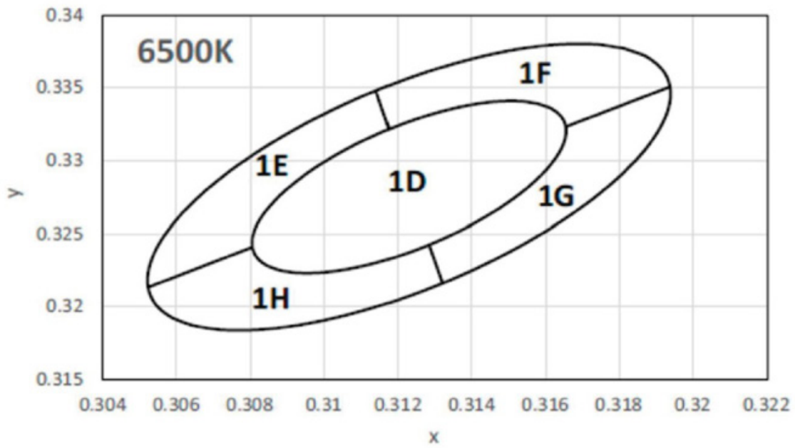
Figure 1i. 1/5 th color bin structure for LUXEON 2835 Commercial Visual Consistency 6500K at specified test current and binning temperature of T_j=25^{\circ}\text{C}
