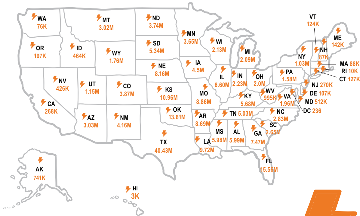
States ranked by total number of lightning events
